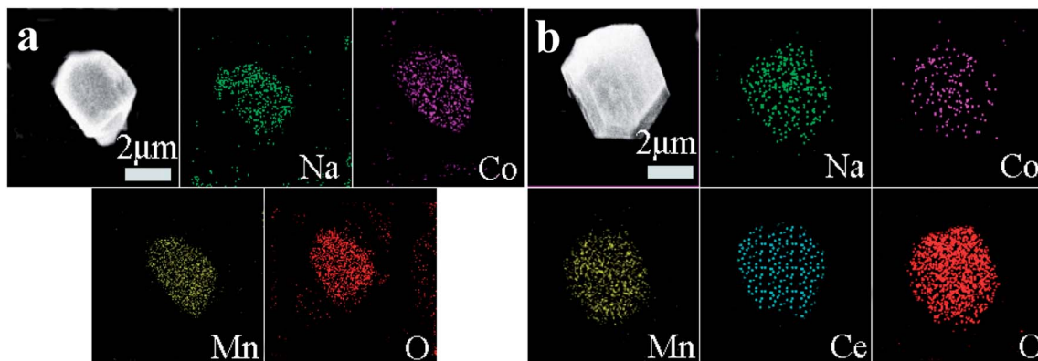
Fig. 4 EDS elementary mapping images of NCMO- x wt% \text{CeO}_2 ( x = 0, 2.00 ) composites, (a) x = 0 , (b) x = 2.00 .
