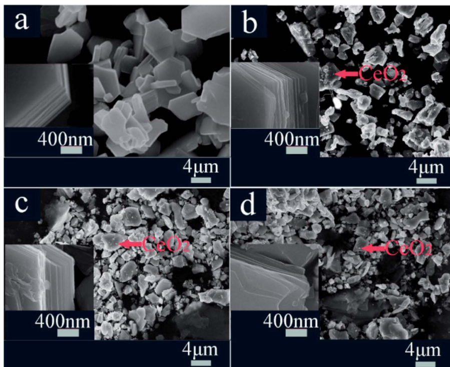
Fig. 3 FESEM images of NCMO- x wt% \text{CeO}_2 ( x = 0, 1.00, 2.00 and 3.00 ) composites, (a) x = 0 , (b) x = 1.00 , (c) x = 2.00 , (d) x = 3.00 .
