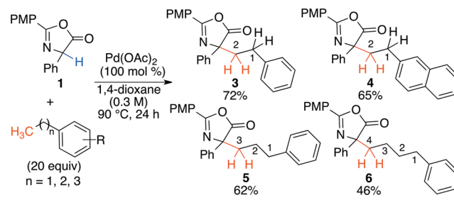
Scheme 3. Selective Primary C–H Activation
