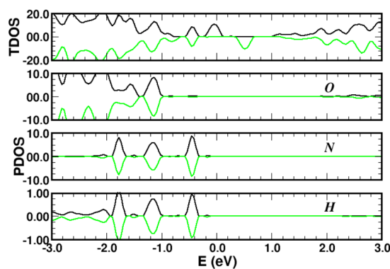
Fig. 16 Total (top panels) and atomic-projected density of states (lower panels) on oxygen (O), hydrogen (H) and nitrogen (N) for four \text{NH}_3 molecules adsorbed on 4SBD-decorated graphene, in arbitrary units.
