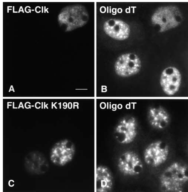
Figure 3. Redistribution of the nuclear speckle stable population of polyA + RNA upon overexpression of Clk/STY. A-431 cells transiently transfected with FLAG-Clk/STY wild-type (A) show redistribution of polyA + RNA (B) to a diffuse nuclear localization. Untransfected cells and cells transfected with FLAG-Clk/STY(K190R) (C) illustrate the typical nuclear speckle localization of stable polyA + RNA (D). Bar, 5 \mu m.
