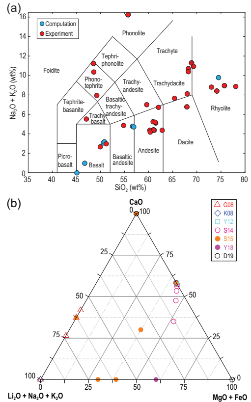
Figure 2. (a) The total alkali-silica (TAS) and (b) CaO–MgO–FeO–Li 2 O+Na 2 O+K 2 O ternary diagrams indicating chemical compositions of silicate melts [15,16,18,19, 21–24,27,28,36,37,39–44,47–56] and carbonate melts [26,30–33,38,45,76], respectively, for which electrical conductivity data reported by experiment and MD simulation were used in this study.
