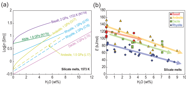
Figure 5. (a) Effect of H 2 O content on electrical conductivity of silicate melts at 1573 K. Data source: N11a [27], L15 [48], L17 [51], G16 [54], C18 [56]. (b) Variation of activation energy ( E in kJ/mol) for silicate melts as a function of H 2 O content. All data are given in Fig. 2a and the Supplementary Data.
