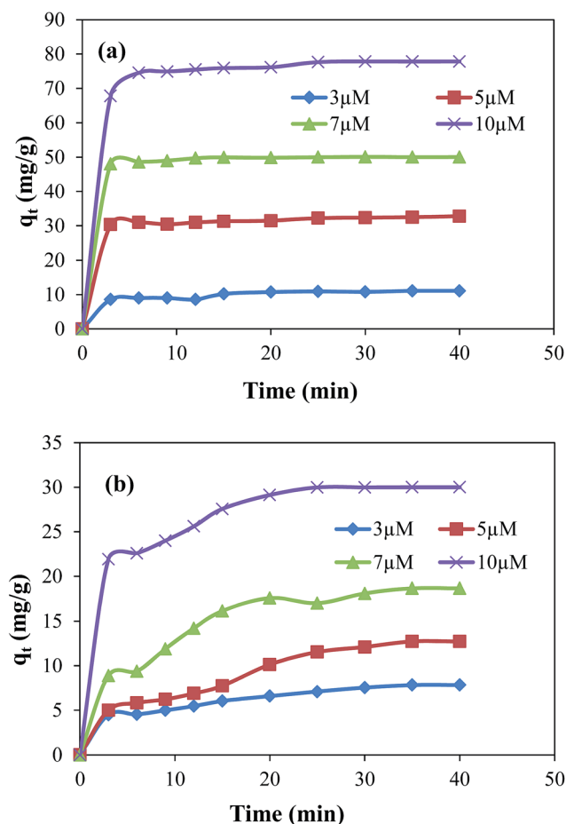
Fig. 3 Effect of initial concentration of dyes on the adsorbed amount of (a) malachite green and (b) ethyl violet on graphene oxide–gold nanocomposite. Reaction conditions; adsorbent = 0.005 g, volume of dyes solution = 50 ml, 100 rpm, 25 °C.
