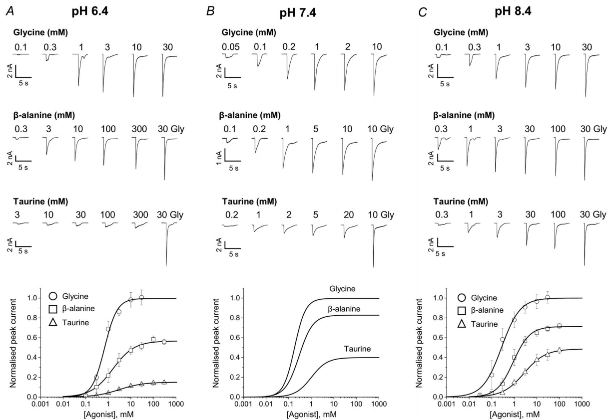
Figure 1. Acidic pH reduces agonist potency and efficacy measured from whole-cell GlyR responses
