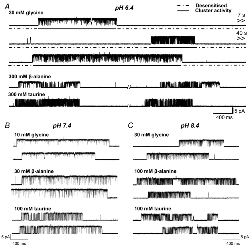
Figure 2. Acidic pH decreases agonist efficacy in zebrafish \alpha 1 GlyR
