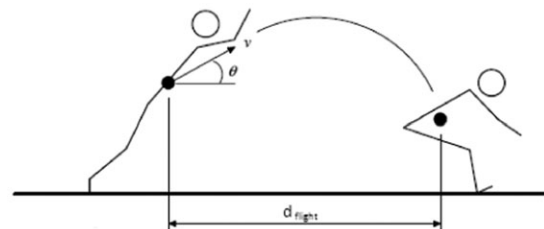
Fig. 1. Depiction of standing horizontal jump, with key terms illustrated. v = take-off speed; \theta = take-off angle, d_{flight} = horizontal distance moved by the centre of mass of the body, h_f = flight height (adapted from Wakai and Linthorne, 2005).
