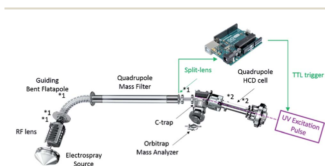
Fig. 1 Schematic diagram of the used Orbitrap EMR instrument to which the UV-laser was coupled. The main parameters altered to optimize detection for large complex subunits and fragments formed thereof by UVPD are displayed with an asterisk: *1 for source-side deceleration of the ions of interest and *2 for trapping in and ejection from the HCD cell (see text for details).
