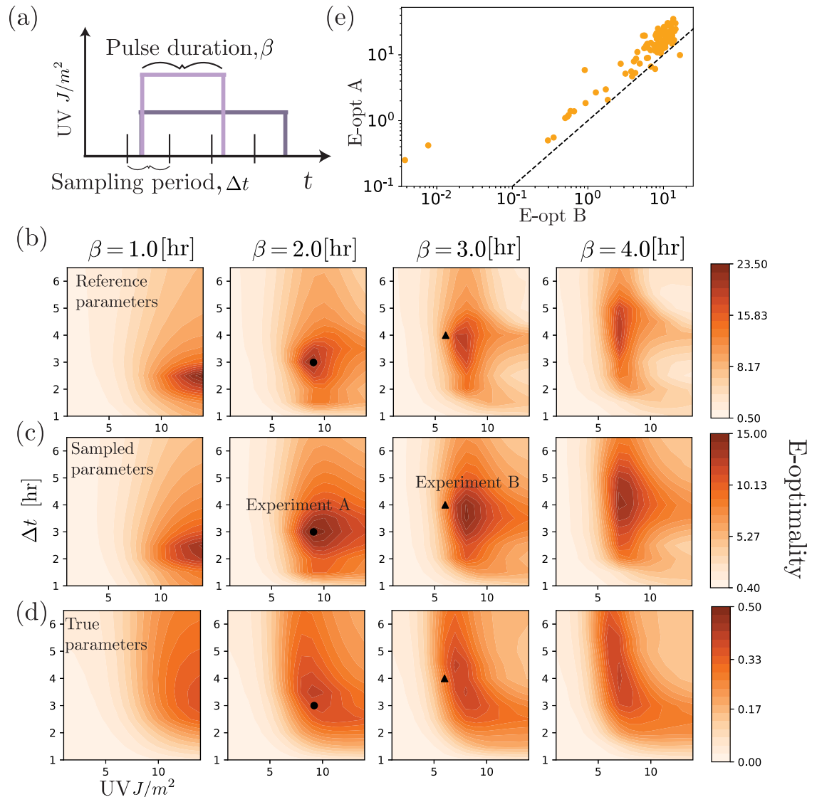
Fig 7. Experiment design for the nonlinear genetic toggle model. (a) Degradation rate of \lambda cI is controlled by UV as shown in Fig 6(a). The magnitude and duration ( \beta ) of UV exposure are free experiment design parameters, along with the time between measurements \Delta t . (b) E-optimality (the smallest eigenvalue of the FIM) versus the 3-dimensional experiment design space, where the FIM is computed using (b) the reference parameter set, (c) by averaging the E-optimality over 100 unique parameter sets and (d) using the “true” parameter values. The black circle is the optimal design chosen according to (c). The black triangle denotes a nearby, but less informative, experiment. (e) For the experiments corresponding to the black circle and triangle in (b-d), E-optimality values are shown for each sampled parameter set.
