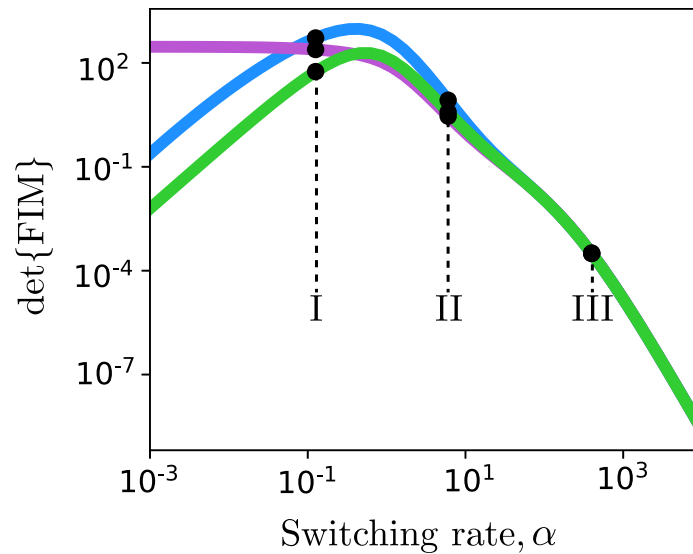
Fig 4. FIM analysis of the bursting gene model. The determinant FIM for the LNA-FIM (purple), FSP-FIM (blue), and SM-FIM (green) as a function of the gene switching rate scale, \alpha . Labels I, II, III correspond to the switch rates for which distributions are plotted in Fig 2(a)–2(c). Parameters are given in the main text and data are assumed to be collected at 10 equally separated time points between 0 and 200 minutes.
