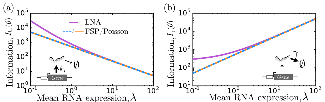
Fig 1. Fisher information for a model of birth and death. The Fisher information for the two model parameters k_r , (a) and \gamma (b) for various values of the mean expression level, \lambda . The analytical form of the FIM for a Gaussian approximation and that computed using Eq 37 (purple line) match to one another. The value computed using the FSP-FIM (blue) matches to the exact form of the analytical Poisson distribution (orange dashed). As \lambda becomes large, all four approaches are consistent.
