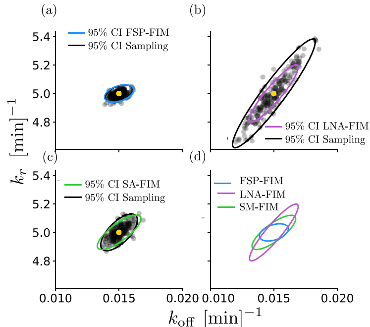
Fig 3. Verification of the FSP-FIM for models with non-Gaussian distributions. The inverse of the FIM is a lower bound on the variance of the MLE estimator. Here, we simulate 200 data sets with 1,000 cells in each data set. We then find the MLE \hat{\theta} (scatter plots) for each, and compare the covariance of these samples to the inverse of the FIM for the (a) FSP-, (b) LNA-, and (c) SM-FIM approaches. Panel (d) shows the FIM matrices for all approximations on the same axes. Simulated data were generated using the parameters given in the main text and at 10 time points evenly distributed between 0 and 200 minutes.
