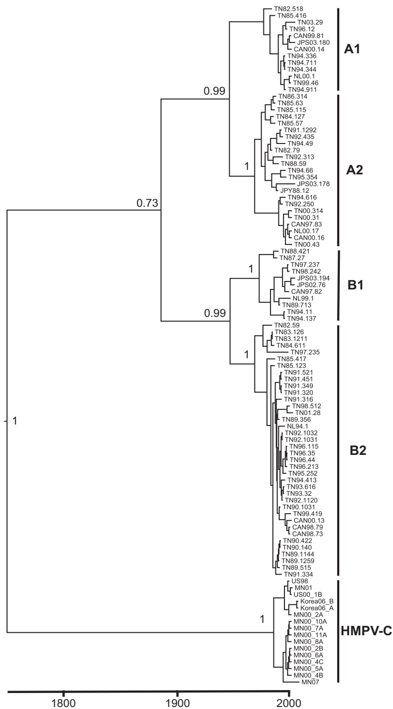
Figure 2 Maximum clade credibility tree of HMPV and AMPV F nucleotide diversity by tMRCA. Phylogenetic analysis of 85 full-length HMPV F nucleotide sequences from Canada (CAN), Japan (JPS or JPY), Tennessee (TN), or the Netherlands (NL) and 16 AMPV F sequences. The first two digits of the HMPV sequence names indicate the year of the isolate. The names of the AMPV sequences indicate geographic origin (US = United States; UK = United Kingdom; MN = Minnesota) and year. The posterior probability of divergence is indicated at each node. Mean TMRCA nodes on the MCC tree differ slightly from those reported in text, although all are contained with the same 95% HPD values. Scale bar represents time in years. Tree was constructed as described in Methods.
