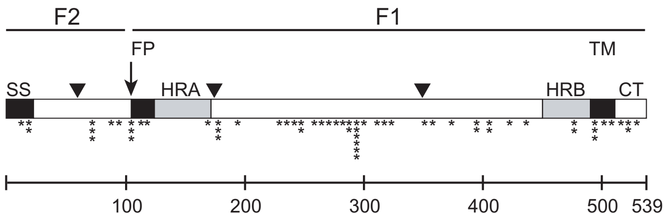
Figure 1 Schematic representation of putative structure and mutation map of human metapneumovirus F protein. SS = signal sequence; FP = fusion peptide; HRA = heptad repeat A; HRB = heptad repeat B; TM = transmembrane domain; and CT = cytoplasmic tail. Arrow indicates cleavage site; arrowheads indicate putative N-glycosylation sites. Amino acid variations are indicated by asterisks, with the number of asterisks representing the number of distinct strains in which the variation was found.
