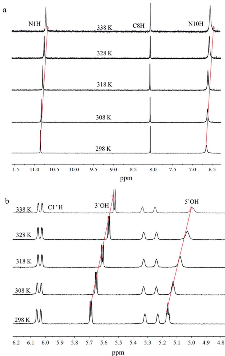
Fig. 8 VT ^1\text{H} NMR spectra of ^F\text{G}_d\text{Ag} recorded from 298 K to 338 K.
