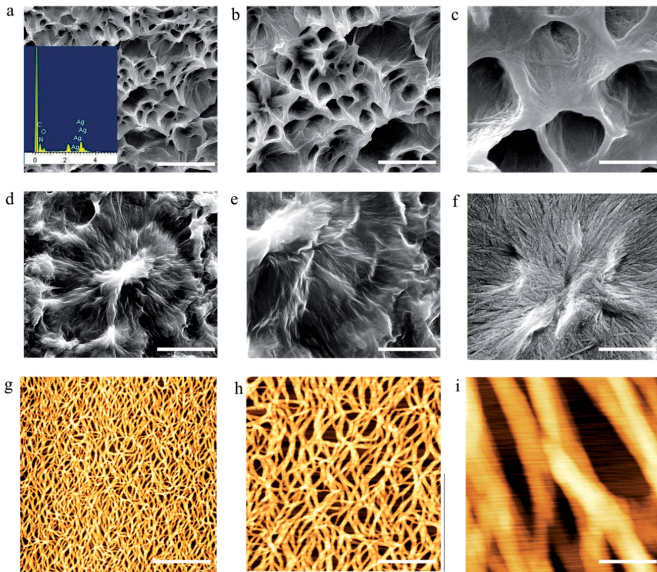
Fig. 7 Microstructures of ^{\text{F}}\text{G}_d hydrogel at the concentration of 0.7% in 0.025 M \text{AgNO}_3 solution. (a–f) SEM images of ^{\text{F}}\text{G}_d hydrogel. (g–i) AFM images of ^{\text{F}}\text{G}_d hydrogel. Scale bars: 5 \mu\text{m} (a and d), 1.5 \mu\text{m} (b and e), 500 nm (c and f), 1.5 \mu\text{m} (g), 500 nm (h), and 50 nm (i).
