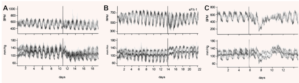
Fig. 5 Representative recordings of heart rate and systolic/diastolic blood pressure. The injection time-point of adenoviruses is indicated by a vertical line on the time axis. Recording of data was estimated for 8–10 days after treatment. Side a shows the treatment with AdveGFP ( 2 \times 10^9 pfu), side b with Adv sFlt-1 ( 3 \times 10^9 pfu) and side c shows the co-treatment with Adv sFlt-1 ( 3 \times 10^9 pfu) and Adv VEGF ( 1 \times 10^8 pfu) for rescue experiments. Indicated is the heart rate (HR) in beats per min (BPM, upper panel) and the systolic (SBP, lower panel, upper graph) and diastolic (DBP lower panel, lower graph), blood pressure in mm Hg.
