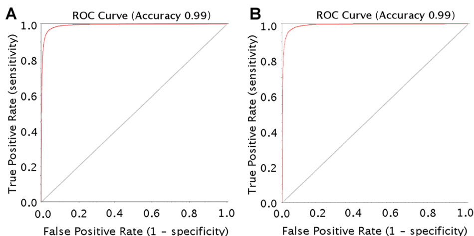
Figure 3 ROC curve and external validation performance (KNIME model). The ROC curves were generated by a Random Forest model ('Tree Ensemble Learner' node). Plot A shows the ROC curve for the out-of-bag classification. Plot B shows the ROC curve for the 80% - 20% stratified cross validation.
