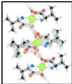
Fig. 2. The packing for (I), viewed down [001], showing hydrogen bonds as dashed lines.
