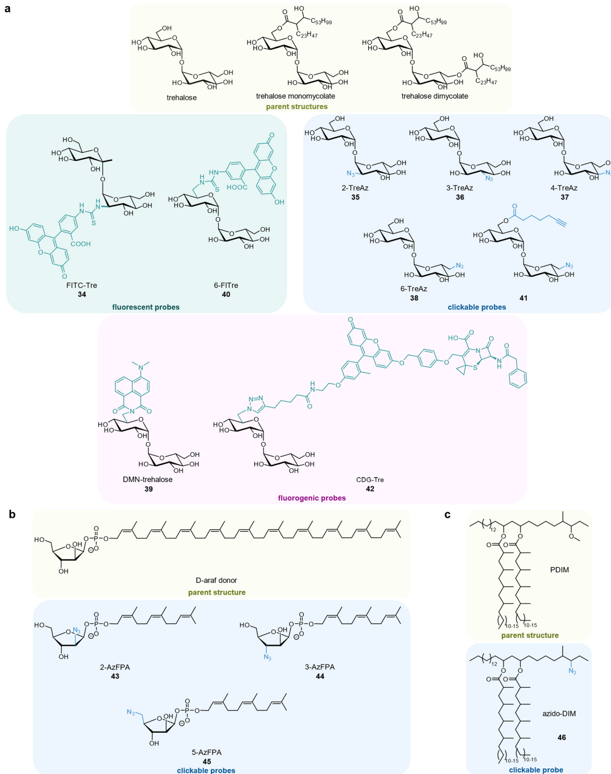
Fig. 6 Mycomembrane components and corresponding probe derivatives. (a) Trehalose-based probes. (b) Arabinose-based probes. (c) Phthiocerol dimycoylate-based probe.
