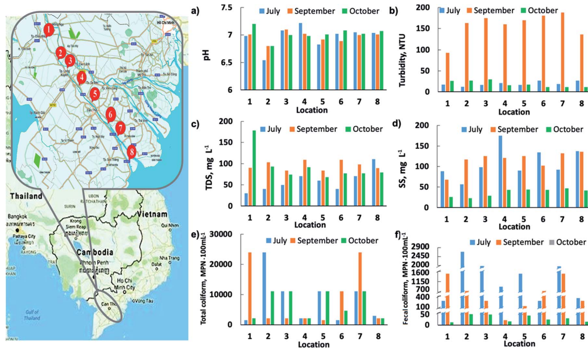
Fig. 5 The sampling locations along the Hau Giang River and preliminary survey of floodwater quality indicators in these locations.
