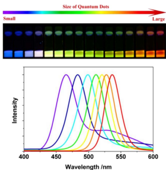
Fig. 2 Emission colors and photoluminescence spectra of QDs with different size. 28
