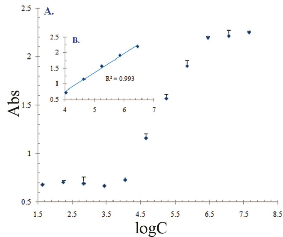
Figure 6. The double-antibody sandwich ELISA for the determination of B. cereus using rabbit polyclonal antibody (as capture antibody, 18 \mu\text{g}/\text{mL} ) and monoclonal antibody 2D2 (as detecting antibody, 1:1000). 'A' is standard curve of sandwich ELISA. 'B' is linear detection line conserved from 'A', linear regression shows a working range from 1 \times 10^4 to 2.8 \times 10^6 cells/mL ( r^2 = 0.993 ), as in the top left insert. X axle: the absorbance of microwell at 450 nm; Y axle: the log Kow of concentration of B. cereus .
