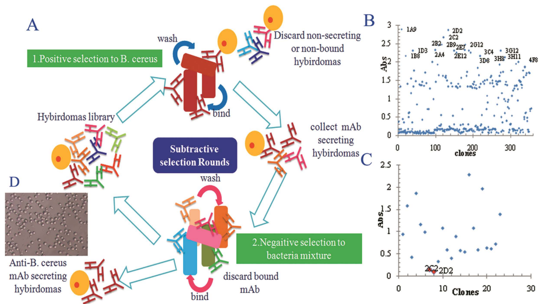
Figure 2. (A) The principle of the subtractive screen. (B) Twenty-three hybridomas were generated against B. cereus by the eighth positive screen. (C) Two non-cross-reactive mAb-secreting hybridomas were generated by the fourth negative selection. (D) The morphology of hybridomas observed under the microscope. All of the selections were conducted by the indirect ELISA.
