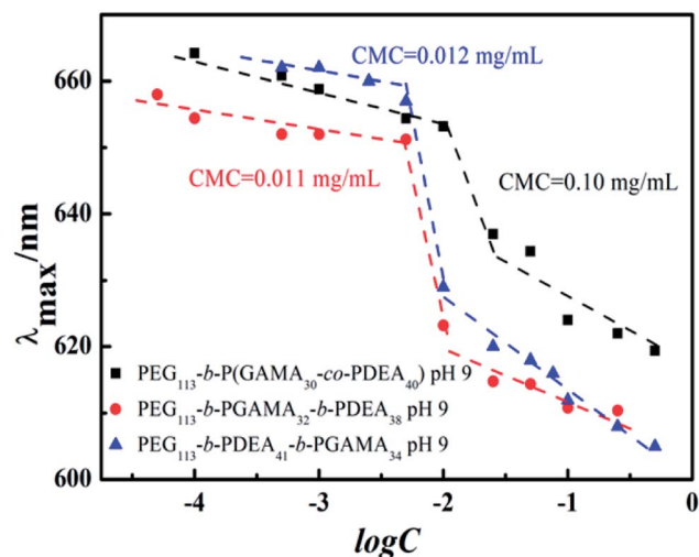
Fig. 3 The dependence of maximum emission wavelength ( \lambda_{\text{max}} ) of Nile Red on the logarithmic concentration of \text{PEG}_{113}\text{-}b\text{-P}(\text{DEA}_{40}\text{-}co\text{-GAMA}_{30}) , \text{PEG}_{113}\text{-}b\text{-PGAMA}_{32}\text{-}b\text{-PDEA}_{38} and \text{PEG}_{113}\text{-}b\text{-PDEA}_{41}\text{-}b\text{-PGAMA}_{34} block glycopolymers.
