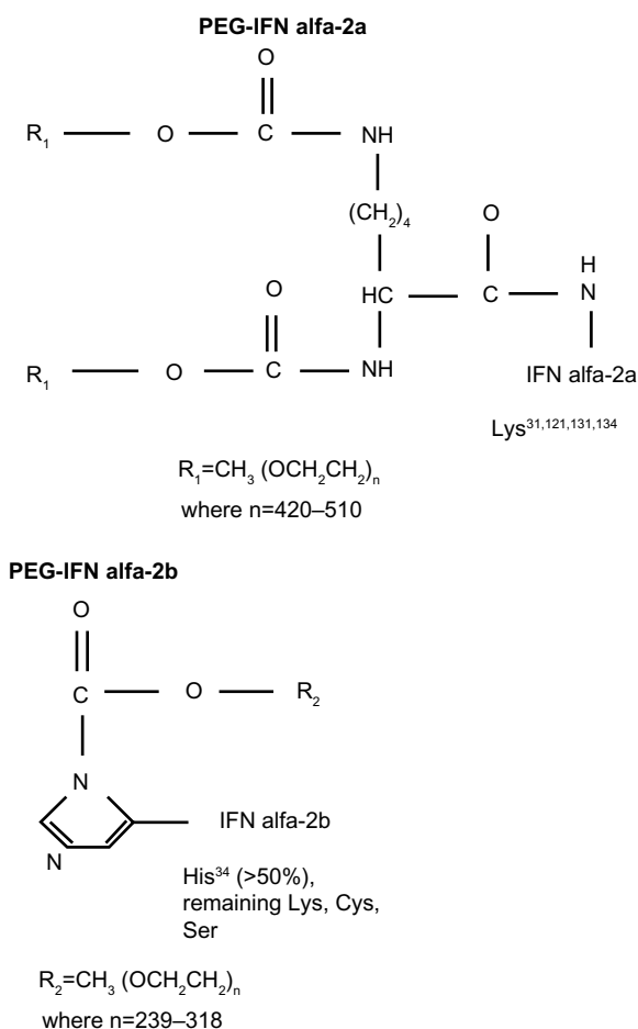
Figure 1 Chemical structure of peginterferon \alpha -2a and \alpha -2b. Abbreviations: PEG-IFN, peginterferon; IFN, interferon; Lys, lysine; His, histidine; Cys, cysteine; Ser, serine.
