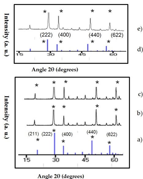
Figure 1. XRD patterns of Y 2 O 3 :Er 3+ /Yb 3+ and Gd 2 O 3 :Er 3+ /Yb 3+ compared with the standard data JCPDS no. 89-5592 [Y 2 O 3 ] and JCPDS no. 88-2165 [Gd 2 O 3 ]. a) JCPDS no. 89-5592 [Y 2 O 3 ] cubic structure, b) Y 2 O 3 :Er 3+ /Yb 3+ (1%, 1%), c) Y 2 O 3 :Er 3+ /Yb 3+ (1%, 10%), d) JCPDS 88-2165:Gd 2 O 3 cubic structure, e) Gd 2 O 3 :Er 3+ /Yb 3+ (1%, 10%). The peaks match in intensity to the JCPDS data; all the samples have cubic structure.
