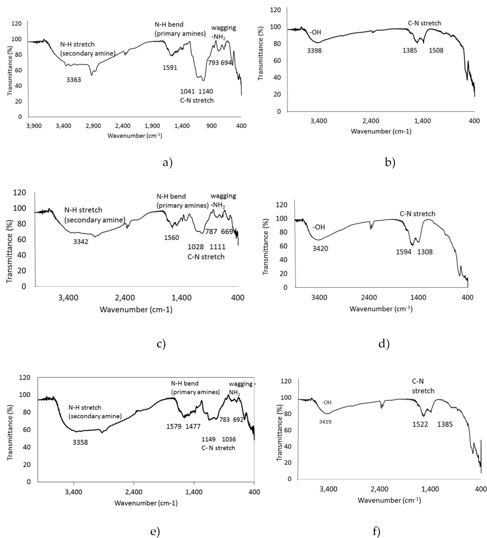
Figure 4. FTIR spectra of aminosilane functionalization UCNPs and bare UCNPs of a) Gd_2O_3:Er^{3+}/Yb^{3+} (1%, 10%) functionalized, b) bare Gd_2O_3:Er^{3+}/Yb^{3+} (1%, 10%), c) Y_2O_3:Er^{3+}/Yb^{3+} (1%, 1%) functionalized, d) bare Y_2O_3:Er^{3+}/Yb^{3+} (1%, 1%), e) Y_2O_3:Er^{3+}/Yb^{3+} (1%, 10%) functionalized and f) bare Y_2O_3:Er^{3+}/Yb^{3+} (1%, 10%). The presence of the amino groups is shown in the N-H stretch of the secondary and primary amines.
