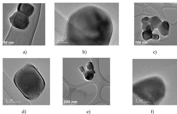
Figure 2. TEM images of (a) bare Y_2O_3:Er^{3+}, Yb^{3+} (1%, 1%); (b) aminosilane functionalization showing the fine silica coating of Er^{3+} 1%, Yb^{3+} 1%; (c) bare Er^{3+} 1%, Yb^{3+} 10%; (d) aminosilane Er^{3+} 1%, Yb^{3+} 10%; (e) bare Gd_2O_3:Er^{3+}, Yb^{3+} and (f) Gd_2O_3:Er^{3+} 1%, Yb^{3+} 10% with aminosilane functionalization.
