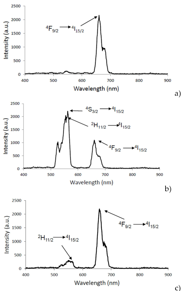
Figure 3. The upconversion emission spectra, under 980 nm excitation for (a) Gd_2O_3:Er^{3+}/Yb^{3+} (1%, 10%), red emission (660-662 nm), for (b) Y_2O_3:Er^{3+}/Yb^{3+} (1%, 1%) green emission (564 nm) in ^4S_{3/2} \rightarrow ^4I_{15/2} transition and (c) Y_2O_3:Er^{3+}/Yb^{3+} (1%, 10%) red emission (661 nm) in ^4F_{9/2} \rightarrow ^4I_{15/2} transition
