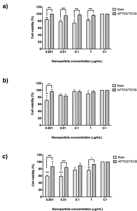
Figure 5. Cell viability assay with 24-hour incubation of bare (pattern bars) and aminosilane (grey bars) UCNPs with HeLa cells. a) Gd_2O_3:Er^{3+}/Yb^{3+} (1%, 10%), b) Y_2O_3:Er^{3+}/Yb^{3+} (1%, 1%) and c) Y_2O_3:Er^{3+}/Yb^{3+} (1%, 10%). Results represent the mean and standard deviation of a threefold independent experiment. * p < 0.05 ; ** p < 0.01 and *** p < 0.001 .
