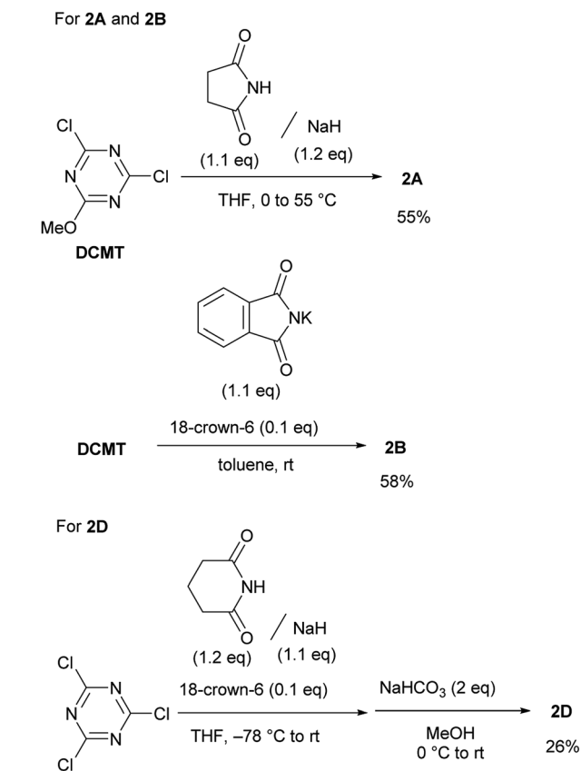
Scheme 2 Synthesis of chlorotriazines ( 2A , 2B , and 2D ).
