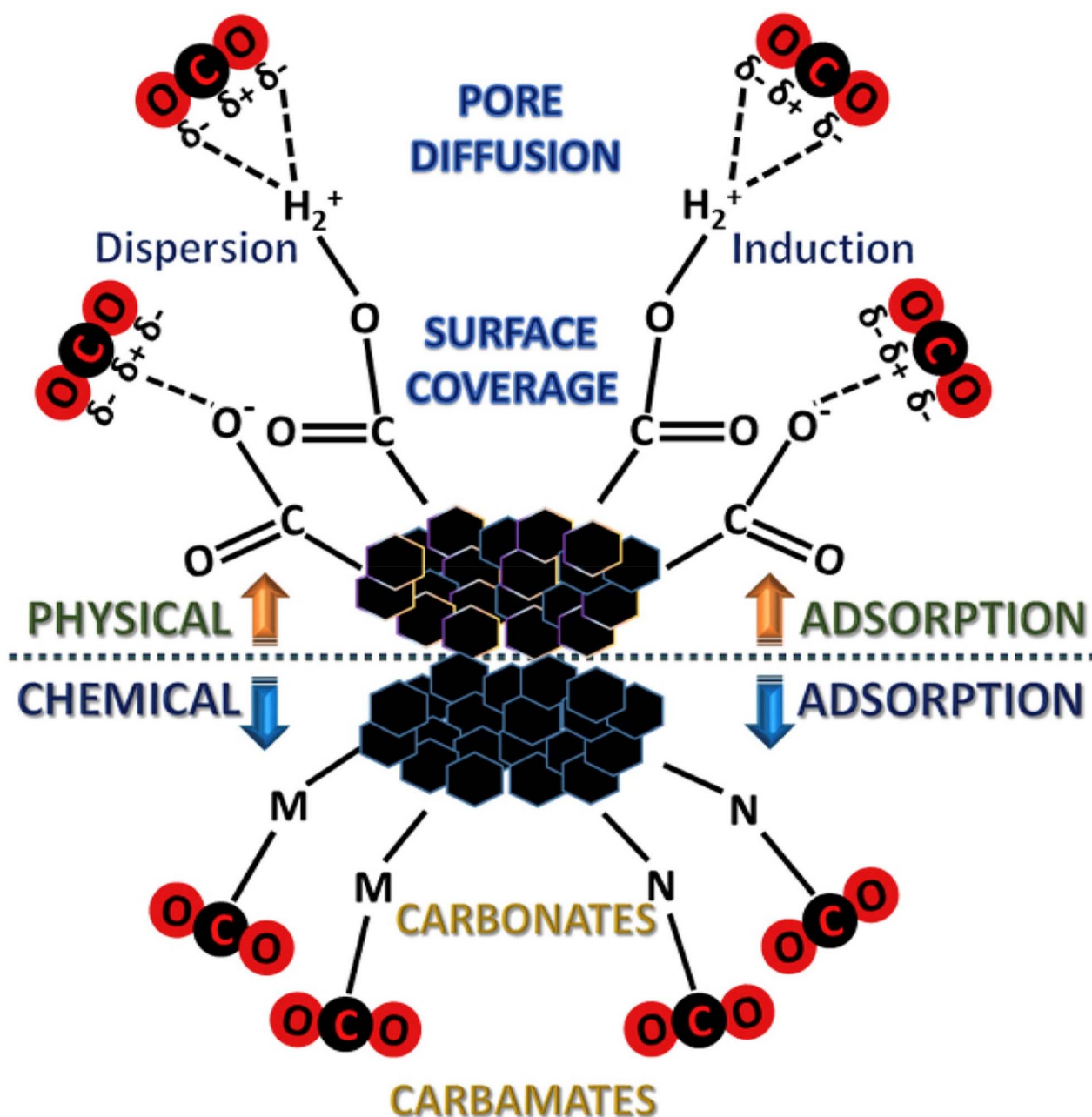
Fig. 3 Physisorption and chemisorption mechanistic process of CO 2 onto the surface of the biomass. 140
