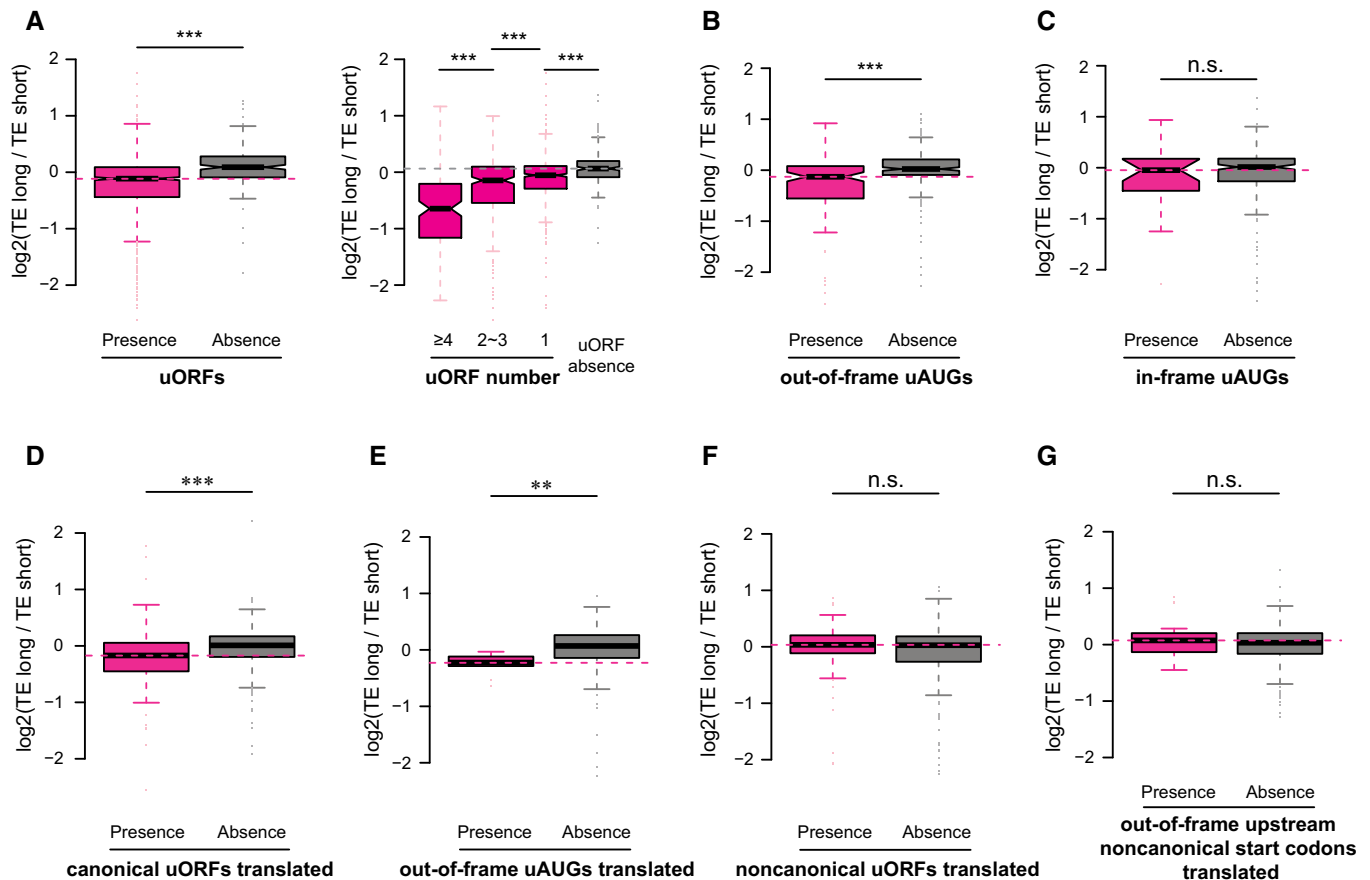
Figure 4. Upstream translation started at AUG negatively affects the main ORF translation.
