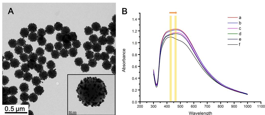
Figure 2. (A) TEM images of single Ag@SiO 2 NPs and distribution of Ag@SiO 2 NPs in EtOH. (B) UV-vis spectra of \beta -CD dimer@Ag@SiO 2 NPs added perylene at (a) 1 \times 10^{-4} M (b) 1 \times 10^{-5} M (c) 1 \times 10^{-6} M and (d) 1 \times 10^{-7} M, and (e) \beta -CD dimer@Ag@SiO 2 NPs in the absence of perylene and (f) Ag@SiO 2 NPs.
