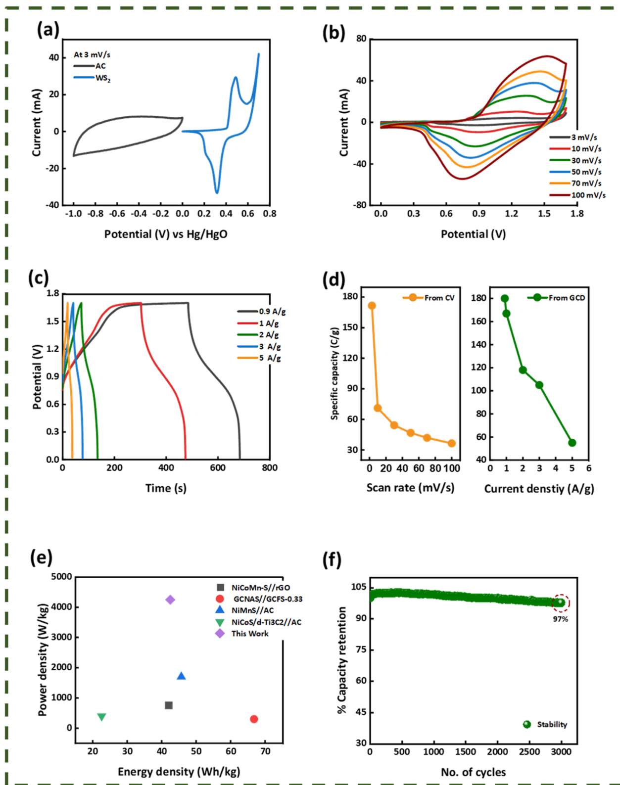
Fig. 8 (a) Comparative CV of activated carbon and WS 2 (W 2 ) at 3 mV s -1 . (b) CV of the WS 2 //AC hybrid device. (c) GCD plot of the WS 2 //AC hybrid device at various current densities. (d) Specific capacities calculated from CV and GCD for the hybrid device. (e) Energy and power density plot of WS 2 //AC. (d) Stability test of the hybrid supercapacitor.
