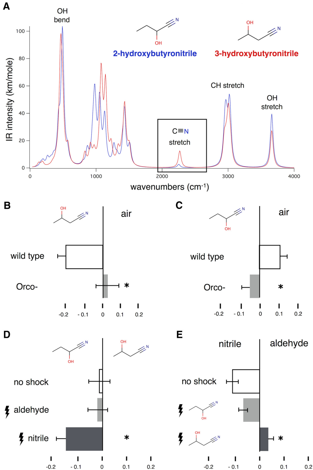
Figure 4. Differential responses to nitrile in the context of different hydroxynitriles. A , Computed I.R spectra of 2- and 3-hydroxybutyronitrile. The location of the -OH group that changes the intensity of the -C≡N stretch (boxed) is shown. Graphs represent the mean relative distribution of flies in the arms of the maze ± SEM after the indicated treatment per condition. Groups of flies were trained by repeated electric footshocks (lightning bolts) in the presence of the indicated odorants per condition. All significance values are calculated relative to the performance of naïve animals (open bars) by LSM contrast analysis and are indicated on the graphs with a single star. B , ANOVA indicated significant differences ( F_{(1,19)} = 7.6564, p < 0.012 ), underlying the significant difference ( p = 0.0076 ) in attraction to 3-hydroxybutyronitrile by wild-type and Orco - mutants. n \geq 7 for all conditions, with a total of 400-500 flies per condition. C , ANOVA indicated significant differences ( F_{(3,39)} = 6014, p < 0.002 ), underlying the significant difference ( p = 0.0136 ) in avoidance of 2-hydroxybutyronitrile by wild-type and Orco - mutants. n \geq 11 for all conditions, with a total of 700-800 flies per condition. D , ANOVA indicated significant differences ( F_{(2,39)} = 3.4240, p < 0.04 ), when flies were differentially
