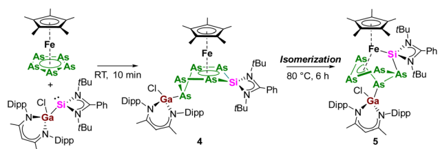
Scheme 3 Reactivity of pentaarsaferrocene [Cp^*Fe(\eta^5-As_5)] towards gallasilylene [L^{Ph}Si-Ga(Cl)L^{BDI}] ( 6 ).
