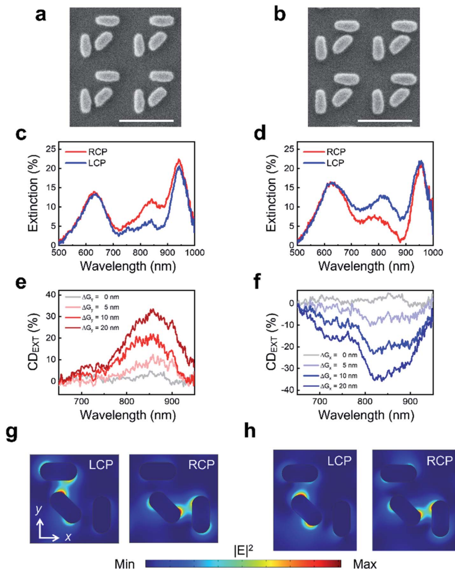
Fig. 3 SEM images of the (a) G_x < G_y ( G_x = 40 nm; G_y = 60 nm) and (b) G_x > G_y ( G_x = 60 nm; G_y = 40 nm) asymmetric nanorod trimers before bonding to the PDMS substrate. The scale bars are 500 nm. Extinction spectra of the trimer metasurface at (c) G_x < G_y as shown in (a), and (d) the counterparts of the trimer metasurface at G_x > G_y as shown in (b). The CD spectra of the trimer metasurface with (e) increasing G_y and (f) increasing G_x . Field profiles of the trimer at (g) G_x = G_y = 40 nm and (h) G_x < G_y under the CP incidence conditions.
