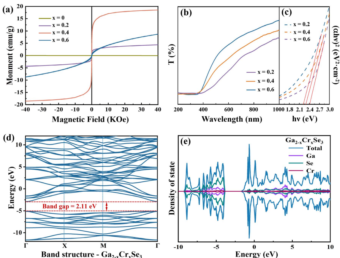
Fig. 6 (a) M - H loops measured at 5 K, (b) transmission spectra, (c) (\alpha hv)^2 - h\nu curves of the \text{Ga}_{2-x}\text{Cr}_x\text{Se}_3 ( 0 \leq x \leq 0.6 ) nanosheets with different Cr concentrations. (d and e) Calculated energy band structure and DOS plot of \text{Ga}_{2-x}\text{Cr}_x\text{Se}_3 sample.
