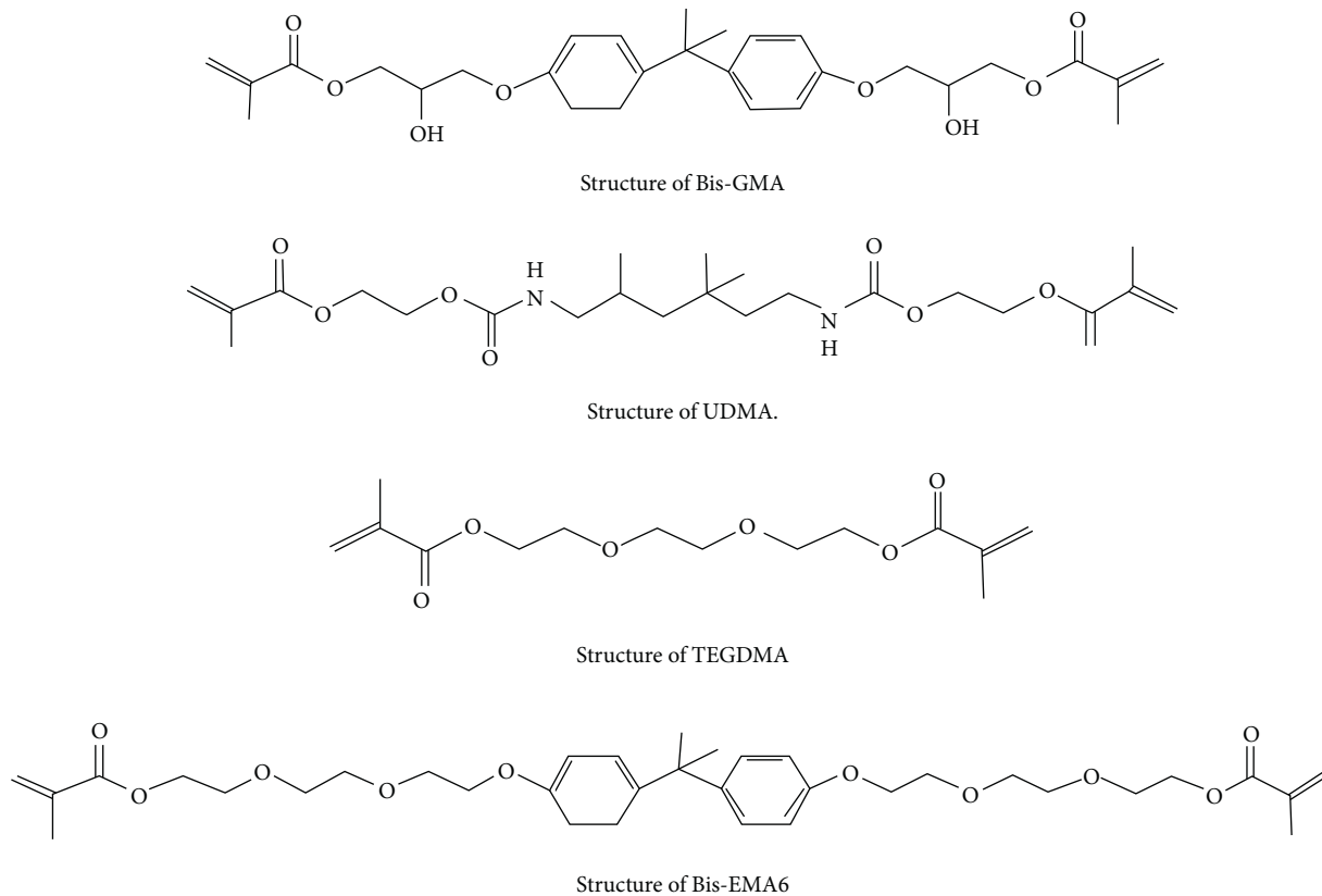
FIGURE 2: Monomer chemical structure measured in this study.
