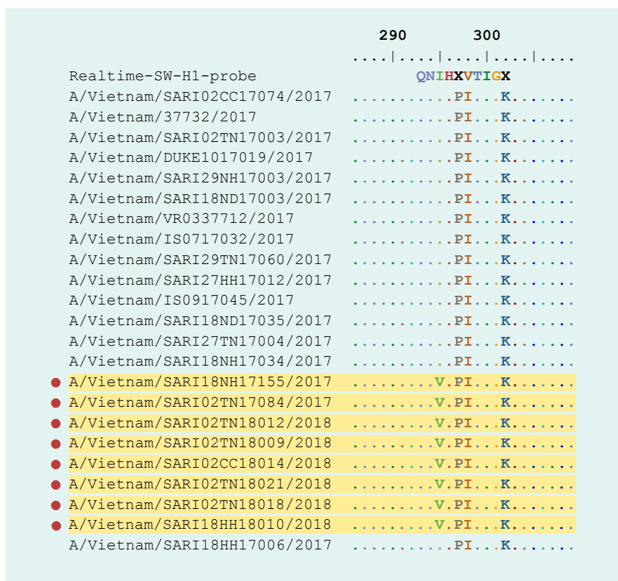
Fig. 3. The substitutions found in the HA protein of influenza A(H1N1)pdm09 compared to the probe sequence
