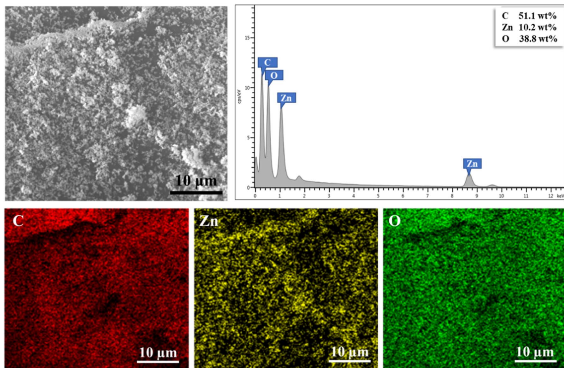
Fig. 9 SEM-EDS micrographs showing the surface of the ZnO/CS + CIT + 2.5% ZIF bead, the corresponding EDS spectrum, and the elemental mapping of C, Zn, and O (magnification 3000 \times ).
