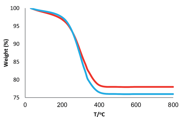
Fig. 10 TGA diagram of CS-FPS/Au NPs. New catalyst (blue), recovered catalyst (red).
