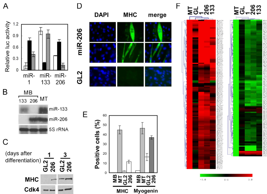
Figure 2. The muscle-specific miRNAs induce the differentiation of muscle cells by regulating many genes. (A) Synthetic oligonucleotides complementary to miR-1, -133, and -206 were inserted downstream of Renilla luciferase ORF in pRL-CMV(MCS) to generate pRL1, pRL133, and pRL206, respectively. Luciferase assays were performed with pRL1 (white bar), pRL133 (black bar), and pRL206 (hatched bar) with the cotransfected RNA duplexes mimicking the miRNAs miR-1, -133, and -206, respectively (x axis). Sequential transfection of each RNA duplex (or miR-125b duplex as a control) and reporter plasmids in GM (serum+) was followed by luciferase assays (20 h after transfection). The y axis indicates relative Renilla luciferase activity, which is normalized as described in Materials and methods. (B) RNase protection assays were performed to measure the level of miR-133 (top) and -206 (middle), in MB transfected with the siRNA duplexes mimicking miR-133 or -206. 5S rRNA was used as a loading control (bottom). RNA from differentiated MTs is shown for comparison. (C) Immunoblots at the indicated days after the serum depletion of C2C12. C2C12 was transfected four times at 24-h intervals with miR-206 or GL2 negative control duplex before serum
