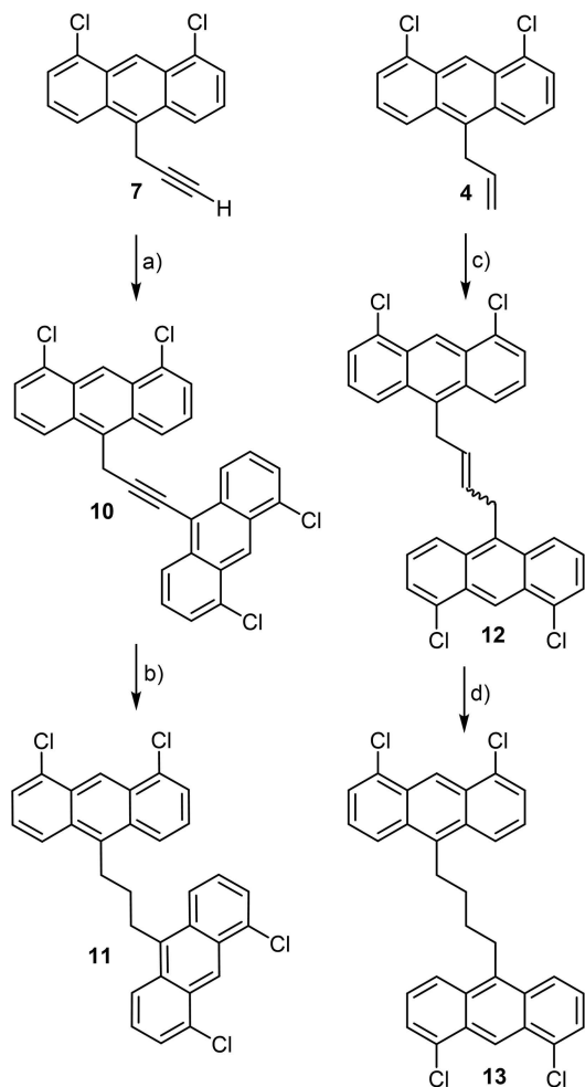
Scheme 4. Syntheses of the bisanthracenylalkanes 11 and 13 . Reagents and conditions: a) 10-bromo-1,8-dichloroanthracene, \text{PdCl}_2(\text{PPh}_3)_2 , CuI, diisopropylamine, reflux, 3d, 33%; b) \text{H}_2 , Pd/C, \text{CH}_2\text{Cl}_2 , 2d, 87%; c) Grubbs' I cat. (5 mol%), \text{CH}_2\text{Cl}_2 , 40^\circ\text{C} , 16 h, 95%; d) \text{H}_2 , Pd/C, \text{CH}_2\text{Cl}_2 , 1d, 63%.
