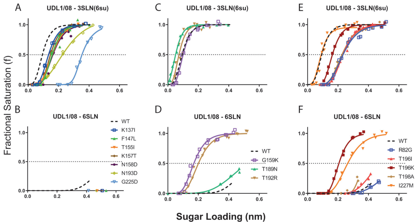
FIG 4 Receptor binding modulation by nonreciprocal mutations in the background of UDL1/08. Bi-layer interferometry was used to determine the receptor-binding profiles of each mutant virus. Binding was measured to three receptor analogues, \alpha 2,6-sialyllactosamine (6SLN), \alpha 2,3-sialyllactosamine (3SLN), and Neu5Ac \alpha 2,3 Gal \beta 1-4(6-HSO 3 )GlcNAc (3SLN[6su]). Dashed black lines show wild-type UDL1/08 binding. Panels indicate binding by mutants that show an avidity reduction (A and B), an increase in avidity (C and D), and changes in receptor-binding preference (E and F). No mutants had any detectable binding to 3SLN.
