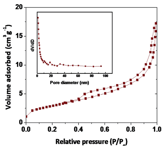
Fig. 6 The BET \text{N}_2 absorption/desorption graph of rhombohedral \text{Fe}_2\text{O}_3 .
