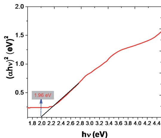
Fig. 7 The \text{Fe}_2\text{O}_3 band-gap calculation by using Tauc plot.
