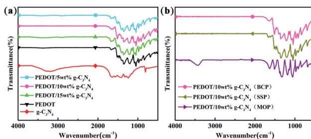
Fig. 1 FTIR spectra of (a) PEDOT (BCP) and PEDOT/ g\text{-C}_3\text{N}_4 nanocomposites with different weight percentages of g\text{-C}_3\text{N}_4 (b) PEDOT/10 wt% g\text{-C}_3\text{N}_4 prepared by different polymerization methods.
