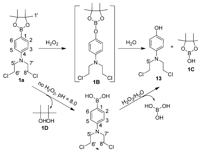
Figure 3. Activation of 1a and 2 by H_2O_2 .
