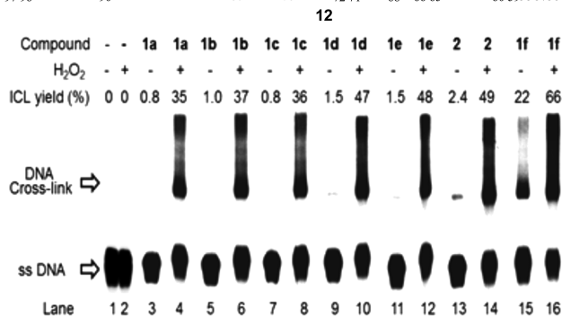
Figure 1. Comparison of the H 2 O 2 -inducible activity and selectivity of 1a–f and 2. Phosphorimage autoradiogram of denaturing PAGE analysis of the cross-linking reaction of DNA duplex 12 in the presence of 1a–f or 2 (1.0 mM) (all reactions were carried out at room temperature).
