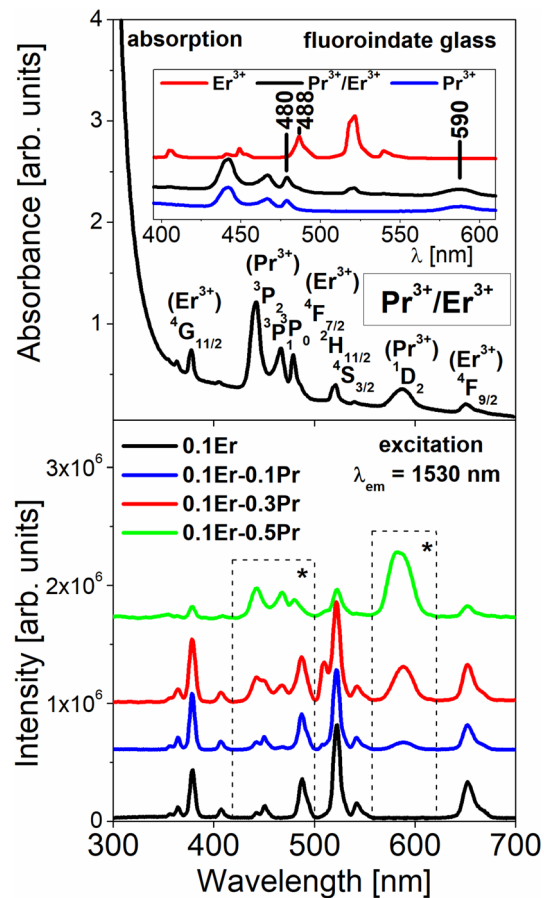
Figure 3. Absorption (top) and excitation (bottom) spectra of fluoroindate glasses co-doped with \text{Pr}^{3+}/\text{Er}^{3+} . The results are compared to the spectra, which were measured for rare earth singly doped glass samples.
