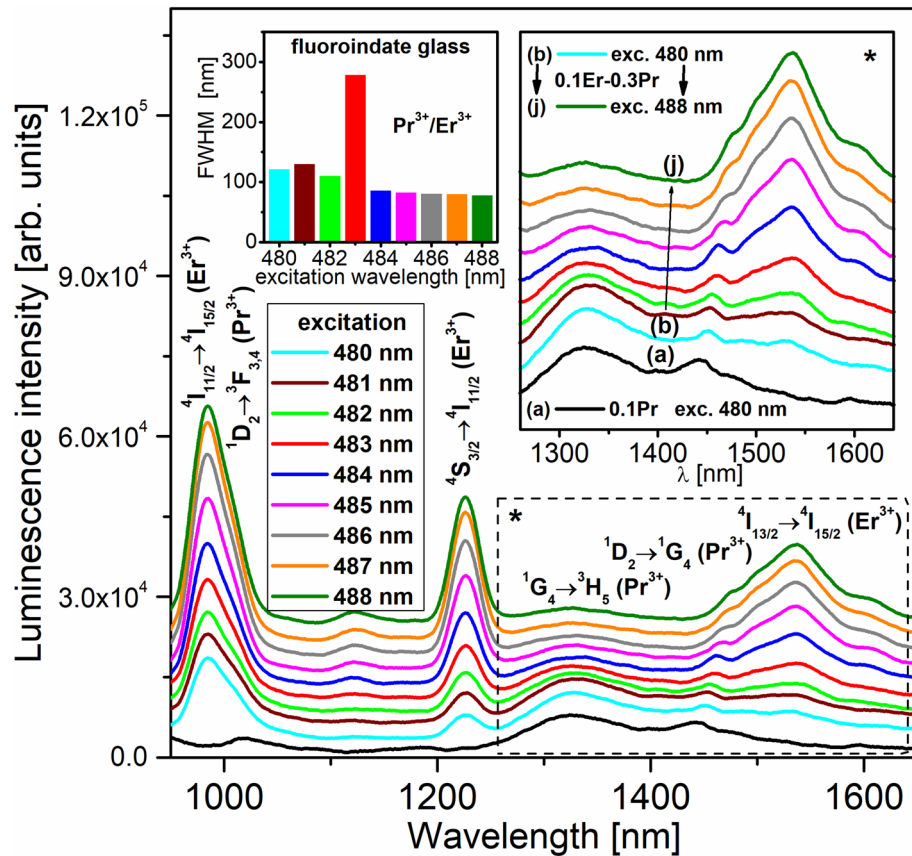
Figure 9. Near-infrared luminescence spectra of fluoroindate glasses co-doped with \text{Pr}^{3+}/\text{Er}^{3+} under selective blue excitation. The inset shows values of FWHM depending on the excitation wavelength.
