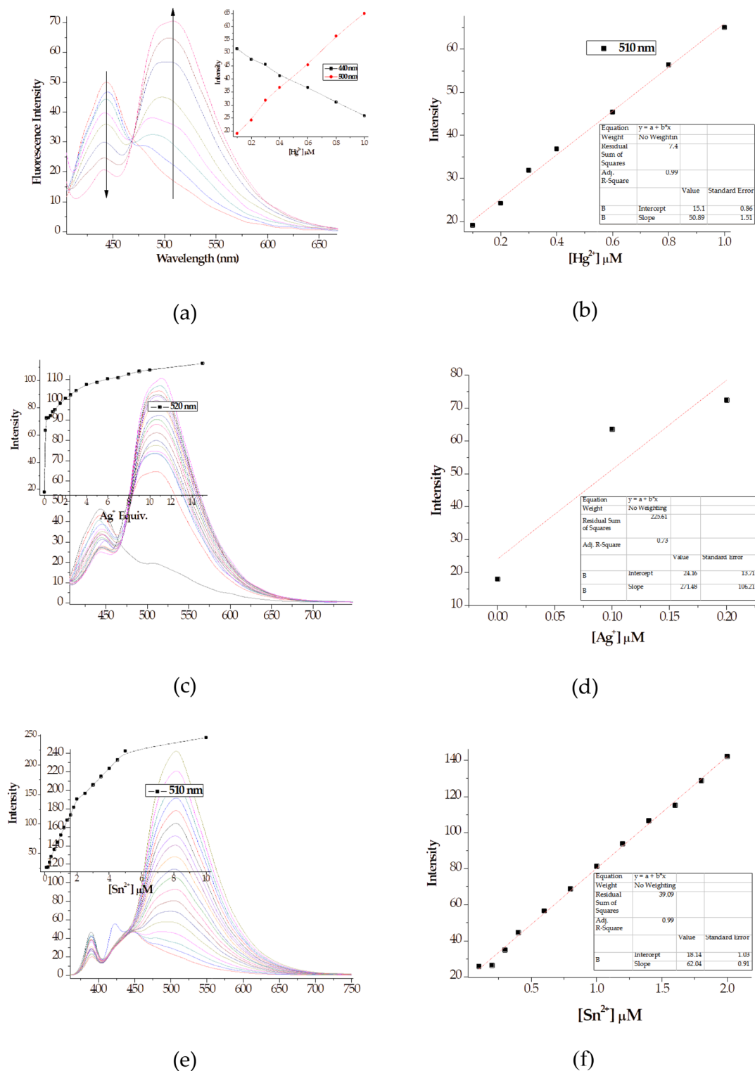
Fig. 12 The fluorescence titration spectra and titration profiles (insets) of M ( 1 \times 10^{-5} M) in DMSO– H_2O , (a) upon the addition of 1 equiv. of Hg^{2+} , (b) fluorescence signals of M to changing conc. of Hg^{2+} (0–1 \mu M ) at 510 nm, (c) upon the addition of 15 equiv. of Ag^+ and (d) fluorescence signals of M to changing conc. of Ag^+ (0–0.3 \mu M ), (e) upon the addition of 10.0 equiv. of Sn^{2+} and (f) fluorescence signals of M to changing conc. of Sn^{2+} (0–2.0 \mu M ), at 510 nm.
