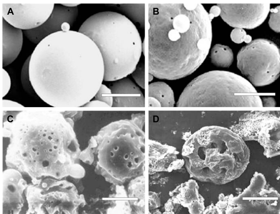
Figure 4 The scanning electron microscope images of bFGF-PLGA MS in shaking flask oscillation group. Notes: (A) Before degradation. B–D are 2, 5, and 8 weeks after degradation, respectively. Scale bars, 5 \mu\text{m} for (A–D). Abbreviation: bFGF-PLGA MS, basic fibroblast growth factor – poly(lactic-co-glycolic-acid) microsphere.
