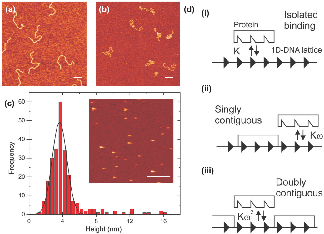
Figure 1. Control experiments. DNA molecules are not observed to cluster in the absence of vTopIB when adsorbed on a mica surface using MgCl 2 (a) or polylysine-coated mica (b). The appearance of the DNA molecules differs as a result of the adsorption processes involved. (c) Histogram of the height of vTopIB molecules measured in buffer in the absence of DNA. The average height of vTopIB in solution is 3.6 \pm 0.9 nm, compatible with a monomeric state of the protein. An AFM image of vTopIB in buffer is shown as an inset in (c). Bar size is 200 nm. (d) Summary of cooperativity theory (19,20). Three different binding events can take place: isolated binding with an association constant K (d, i), singly contiguous binding with an association constant K\omega (d, ii) and doubly contiguous binding with association constant K\omega^2 (d, iii). In our model an isolated binding event is attributed to the formation of an intramolecular node.
