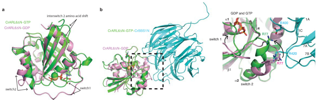
Fig. 4. Nucleotide-dependent conformational changes in CrARL6
