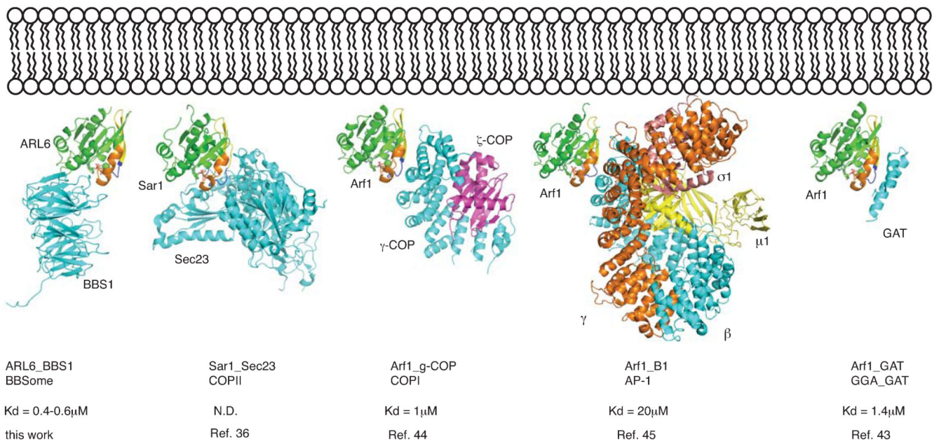
Fig 6. Structural comparison of membrane recruitment of coating complexes by Arf, Sar and Arf-like proteins
