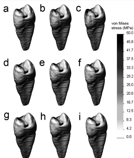
FIGURE 8. Von Mises stress distribution results (A) Model 1: 3D solid tooth model with mesio-occlusal-distal (MOD) cavity with 3.0 mm wall thickness, without cusp reduction; (B) Model 2: 3D solid tooth model with MOD cavity with 2.25 mm wall thickness, without cusp reduction; (C) Model 3: 3D solid tooth model with MOD cavity with 1.5 mm wall thickness, without cusp reduction; (D) Model 4: 3D solid tooth model with MOD cavity with 3.0 mm wall thickness and 2.0 mm palatal cusp reduction; (E) Model 5: 3D solid tooth model with MOD cavity with 2.25 mm wall thickness and 2.0 mm palatal cusp reduction; (F) Model 6: 3D solid tooth model with MOD cavity with 1.5 mm wall thickness and 2.0 mm palatal cusp reduction; (G) Model 7: 3D solid tooth model with MOD cavity with 3.0 mm wall thickness and 2.0 mm palatal and buccal cusp reduction; (H) Model 8: 3D solid tooth model with MOD cavity with 2.25 mm wall thickness and 2.0 mm palatal and buccal cusp reduction; (I) Model 9: 3D solid tooth model with MOD cavity with 1.5 mm wall thickness and 2.0 mm palatal and buccal cusp reduction.
