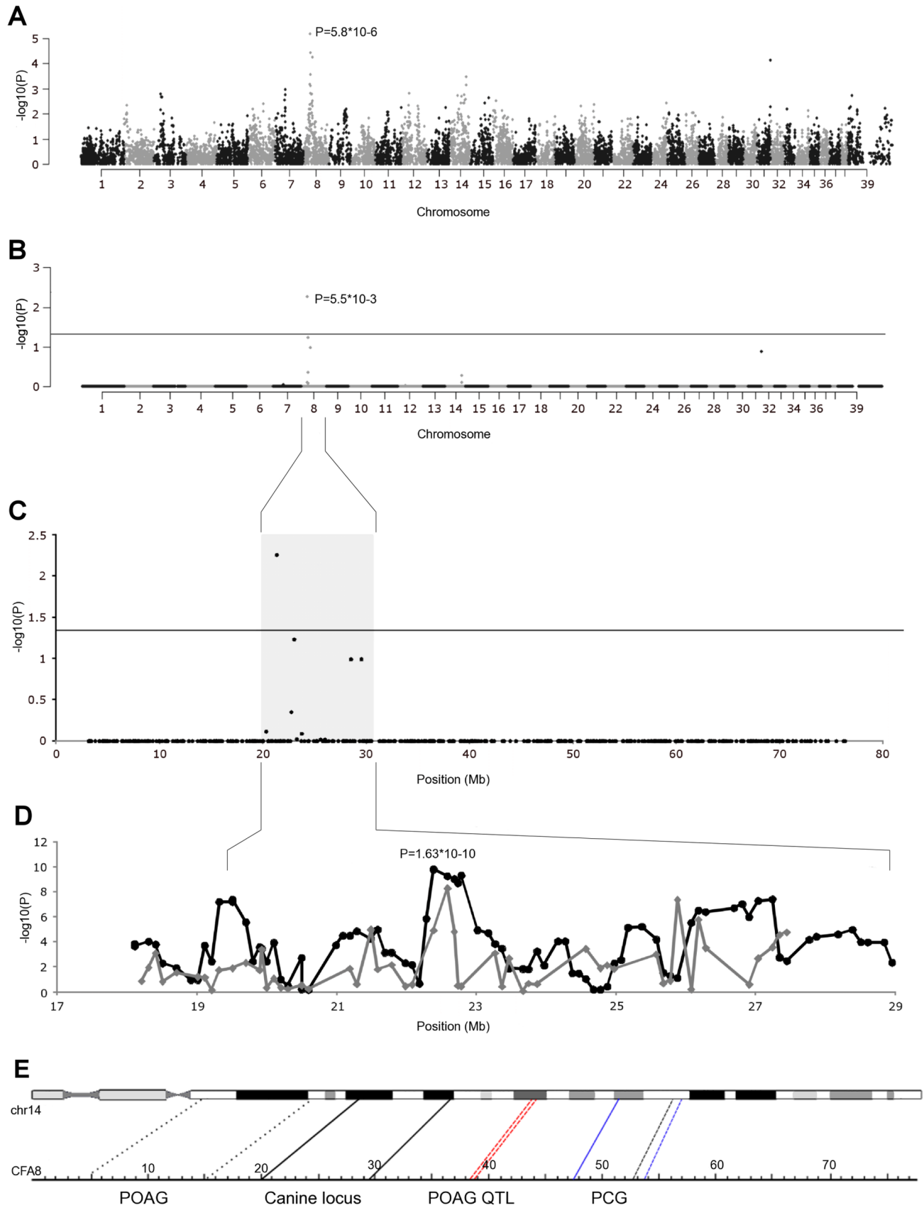
Figure 1. Genome wide association analysis. A) A Manhattan plot of genome-wide case-control association analysis performed using 23 cases and 23 controls. B) Results of the genome-wide association analysis after 50,000 permutations. A significant association was identified on CFA8
