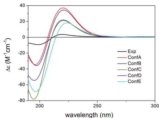
Fig. 11 Experimental ECD spectrum of 3 in MeCN compared with the Boltzmann-weighted B3LYP/TZVP PCM/MeCN ECD spectra of the individual five lowest-energy CAM-B3LYP/TZVP PCM/MeCN conformers of (1 R ,2 S ,3 R ,4 S ,5 S ,9 S ,10 R ,13 R ,17 R ,30 R )- 3 .
