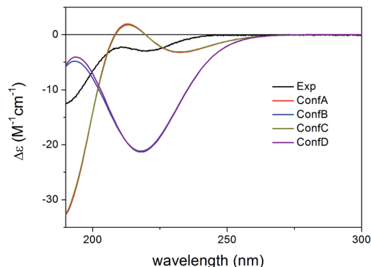
Fig. 17 Experimental ECD spectrum of 6 in MeCN compared with the BH&HLYP/TZVP PCM/MeCN ECD spectra of the individual four lowest-energy CAM-B3LYP/TZVP PCM/MeCN conformers of (1 R ,2 S ,3 R ,4 S ,5 S ,9 S ,10 R ,13 R ,14 S ,17 R )- 6 . Experimental ECD spectrum of 6 was reproduced with permission from ref. 16.
