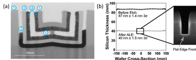
Fig. 6 (a) Example of etch selectivity in thermal ALE at 250 °C. Materials are (1) SiN , (2) HfO_2 , (3) SiO_2 , (4) TiN , and (5) Al_2O_3 . No measurable removal in SiN , SiO_2 , and TiN was detected after 1000 ALE cycles. 46 (b) Plasma-assisted ALE results showing characteristic ALE benefits with excellent depth uniformity across the wafer and flat silicon etch front on the feature. 26
